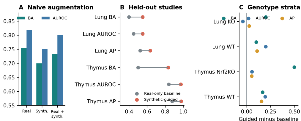
Figure S5. Downstream utility of generated expression. (A) Direct pooled augmentation on the locked real test. (B) Fixed synthetic-guided policies in independently held-out lung and thymus accessions. (C) Guided-minus-baseline metric changes after post-hoc genotype stratification. Thymus improved uniformly; lung knockout AUROC declined.
