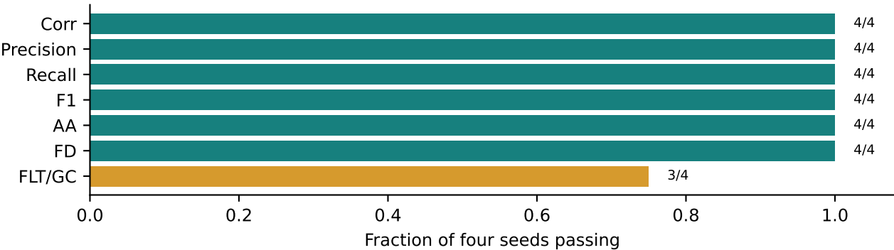
C DDIM repeat performance
