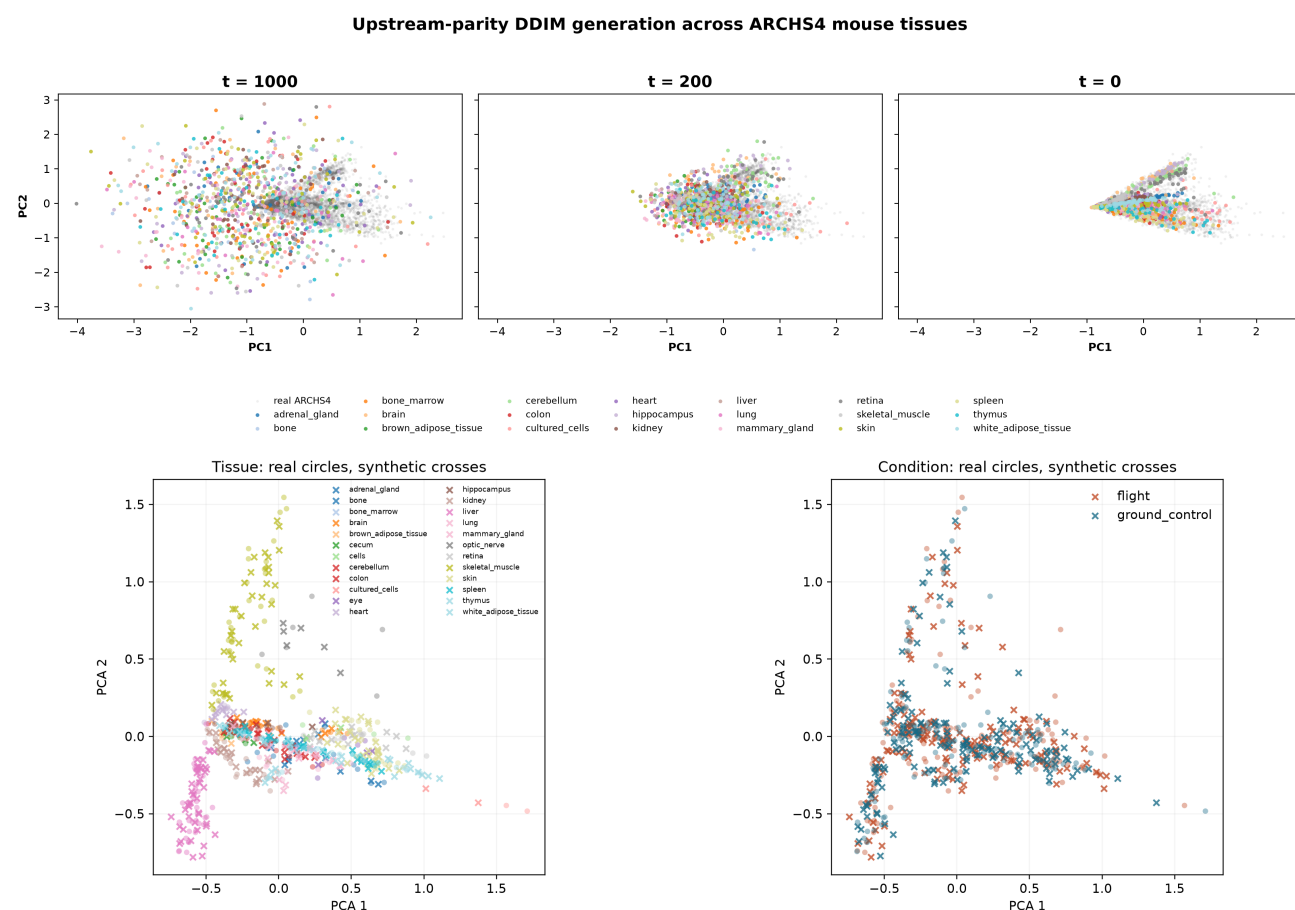
Figure 3. Diffusion generation across reference pretraining and OSDR adaptation. Top: ARCHS4 tissue-conditioned profiles at DDIM timesteps 1,000, 200, and 0 in a PCA space fitted to real reference expression; gray points are real ARCHS4 profiles and colors identify generated tissue conditions. Bottom: locked OSDR profiles for generation seed 5020; circles denote real profiles and crosses denote generated profiles, colored by tissue on the left and flight condition on the right. PCA views are descriptive and do not replace the quantitative validation gates.
