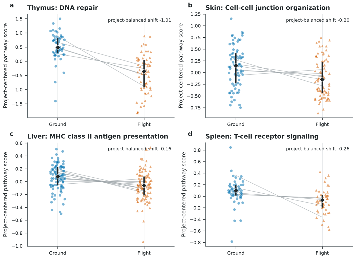
Figure S9. Sample-level distributions for representative retained programs. Individual OSD samples are shown after decoder orientation and centering within OSD accession. Blue circles are ground controls and orange triangles are flight samples; gray segments connect condition means within a project. Black diamonds and bars show the condition median and interquartile range. The annotated shift is the primary project-balanced expiMap effect, which is not estimated by treating individual points as independent. Skin uses the broad flight label; protocol-defined contrasts are shown in Figure 5.
