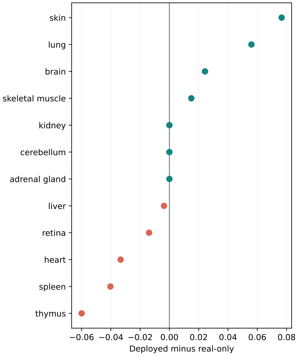
Balanced accuracy
