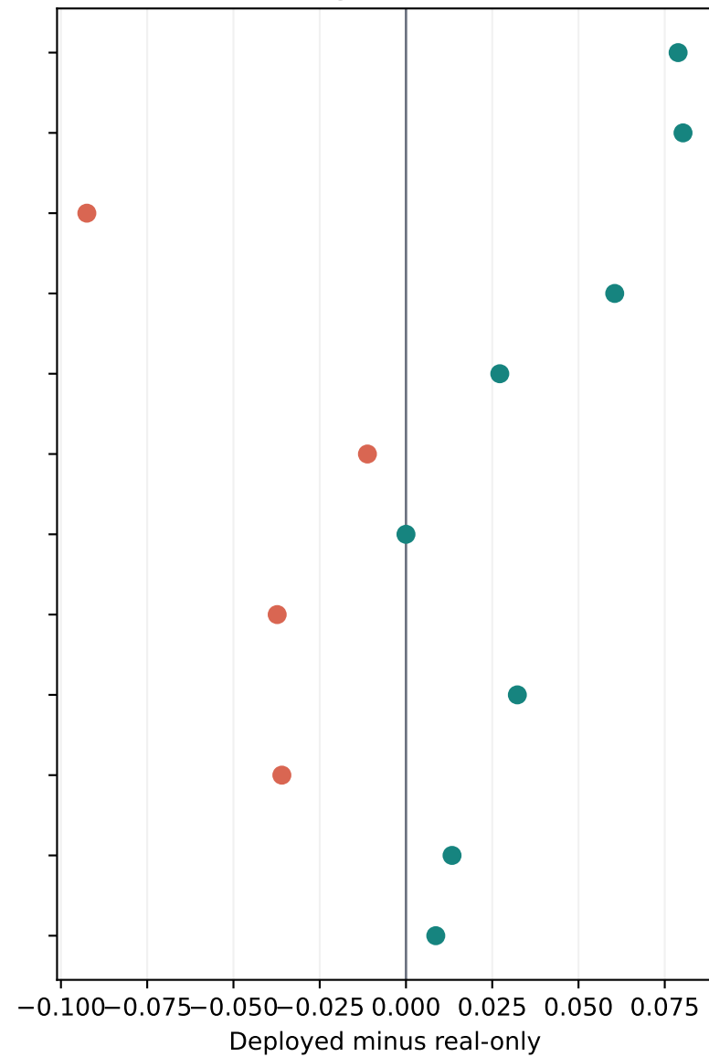
Average precision
