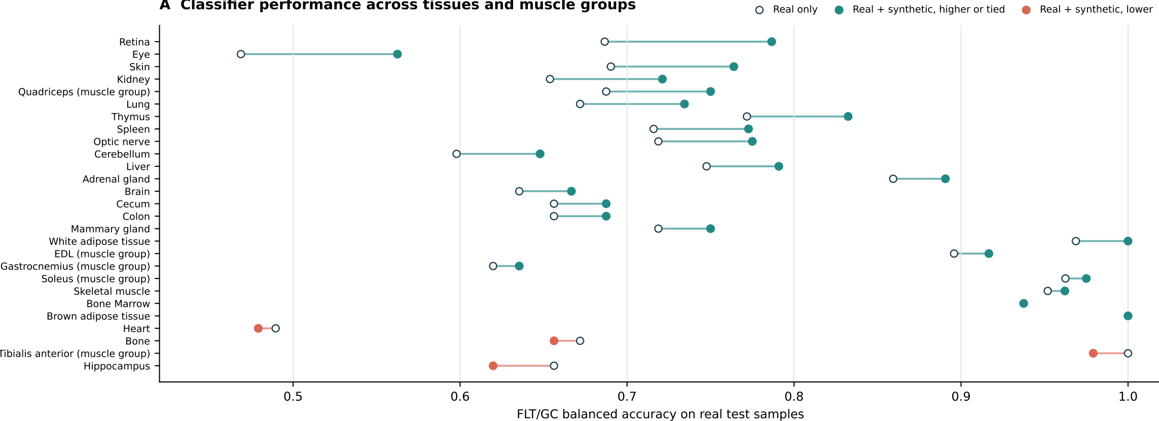
A Classifier performance across tissues and muscle groups
