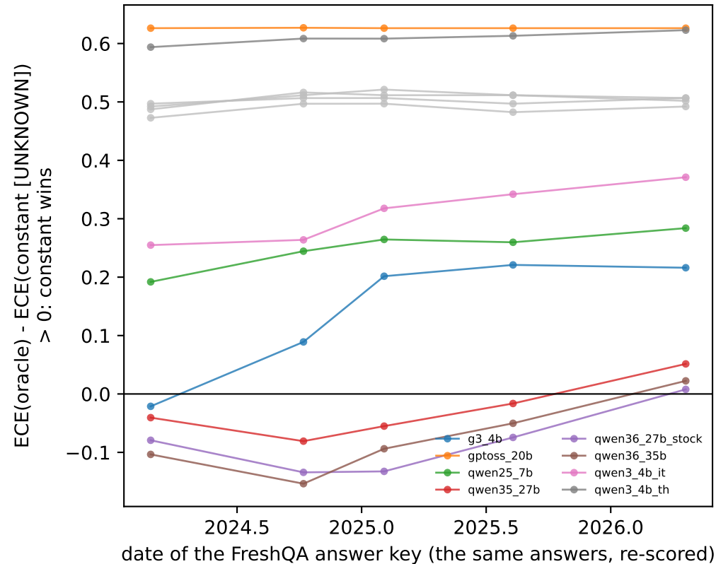
B. FreshQA: the constant overtakes the oracle as the key moves past the model's knowledge (grey: hedge-trained Qwen2.5-7B adapters)
