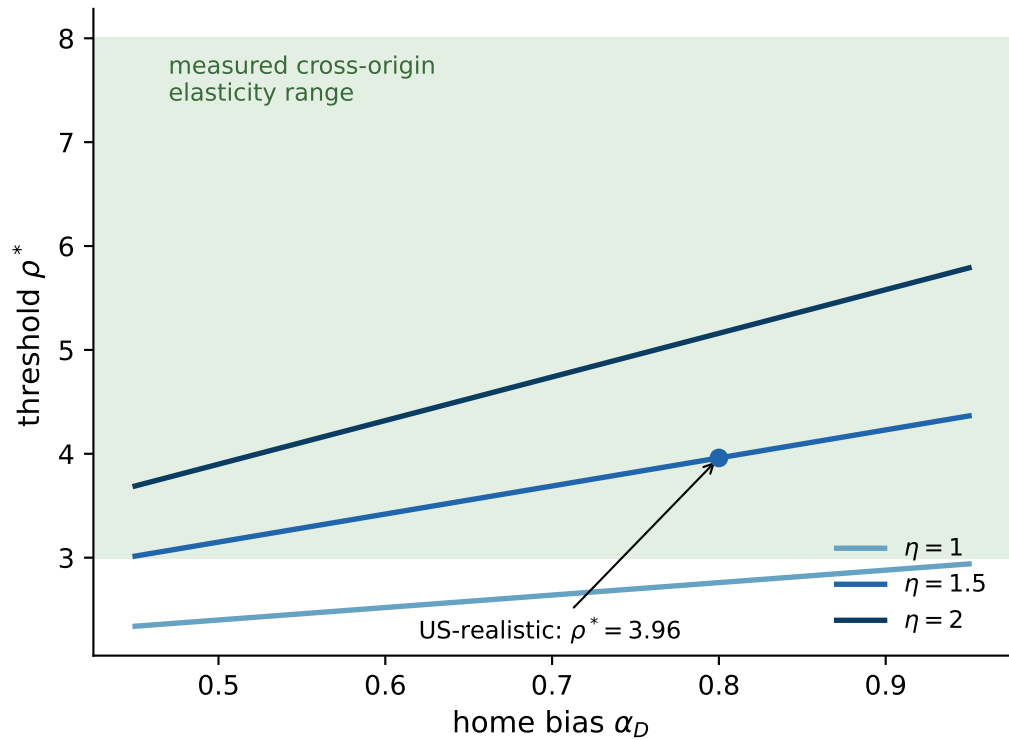
(b) \rho^* = 3[1 + \alpha_D(\eta - 1) - \alpha_T(1 - \alpha_D)]
