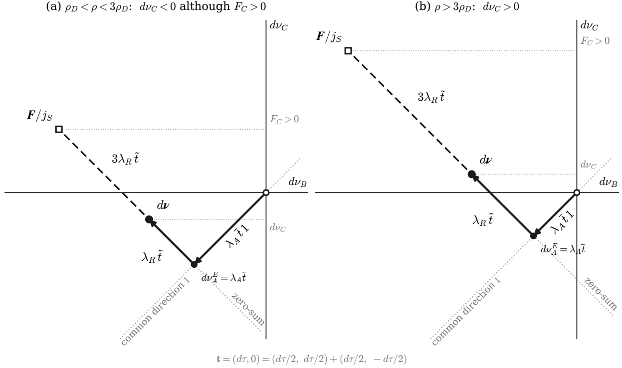
Figure 2: Average protection and relative treatment under a unilateral tariff at N = 3 . Solid arrows decompose the equilibrium response d\mathbf{v} ; the dashed arrow extends the relative-treatment component to \mathbf{F}/j_S . Drawn at \alpha_D = 0.7 , \alpha_T = 0.6 , \eta = 1.5 and \mathbf{t} = (1, 0) , with \rho = 2.2 in panel (a) and \rho = 5 in panel (b).
