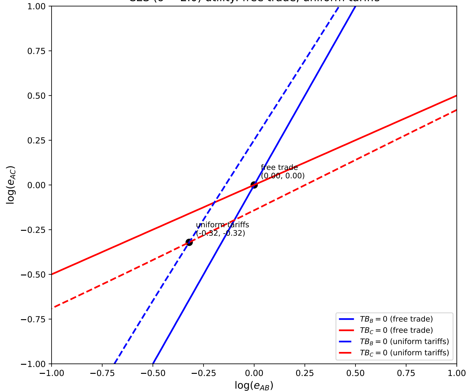
CES ( \sigma = 2.0 ) utility: free trade, uniform tariffs
