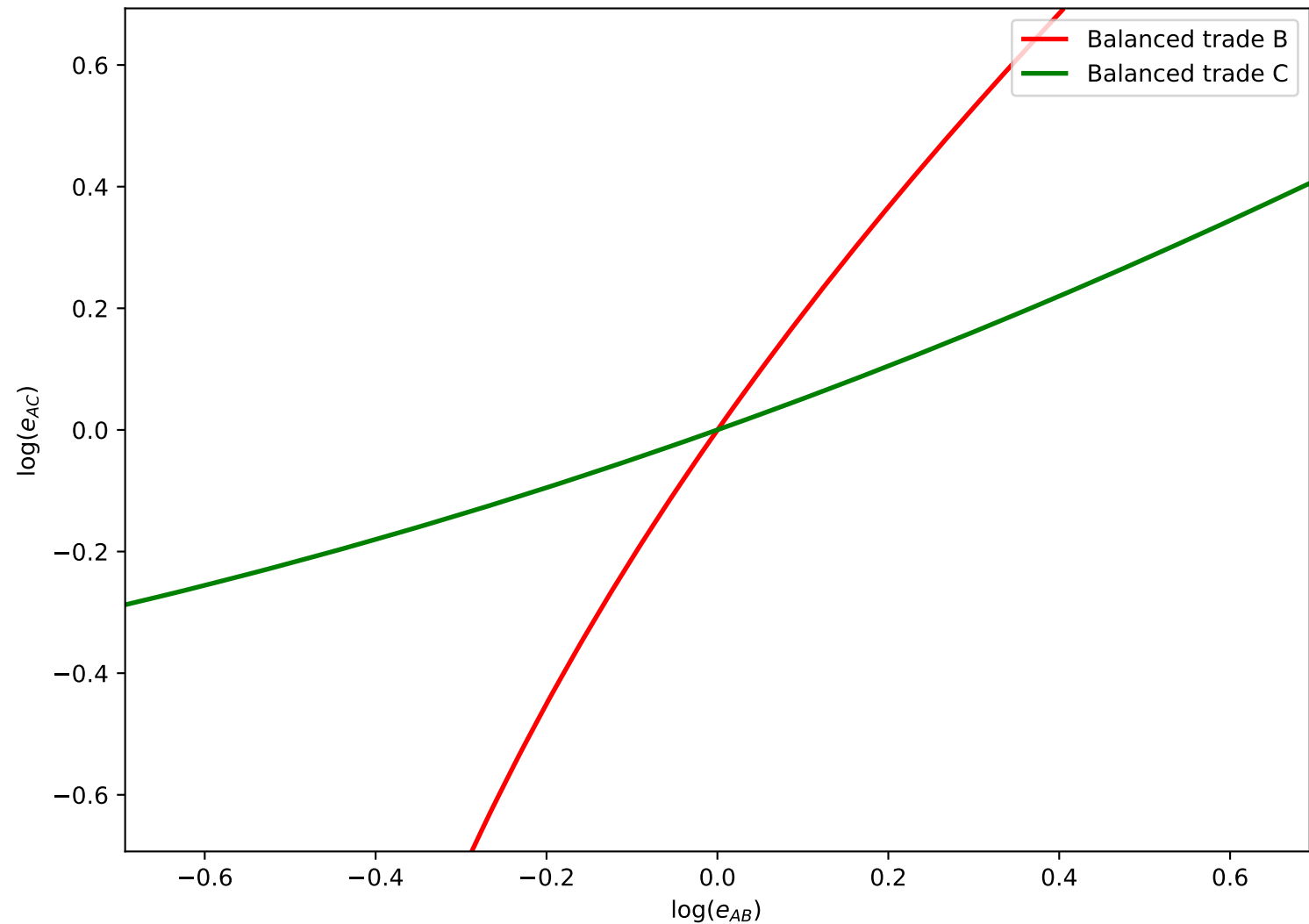
3c2s1f model: balanced trade loci for B and C
