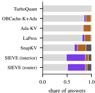
(c) How answers fail (Llama, 128k)
