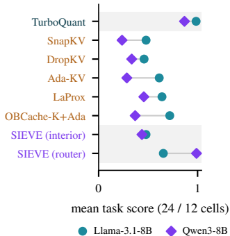
(a) The winner depends on the model
