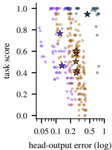
(b) Output error vs. task score within-cell \rho : -0.05 (8 methods); 8k run: -0.36 (12)
