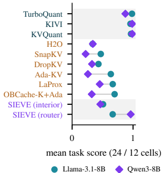
(a) The winner depends on the model
