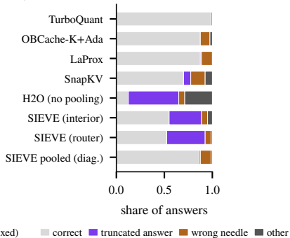
(c) How answers fail (Llama, 128k)
