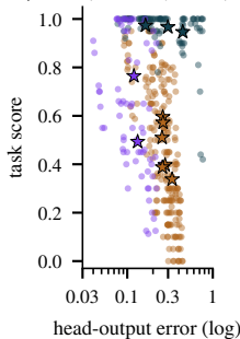
(b) Output error vs. task score within-cell \rho : -0.16 (12 methods); -0.38 (8 token-selective)
