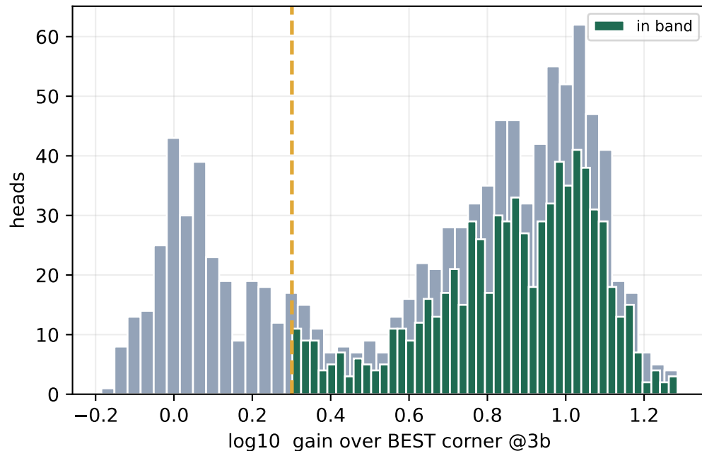
Where the model's heads actually fall
