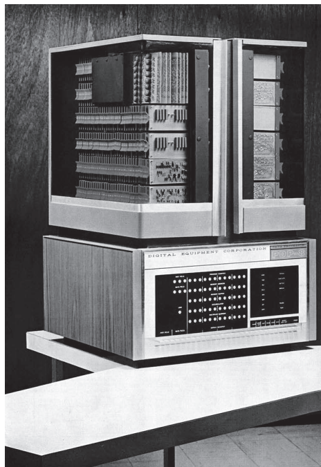
Figure 38 In the mid-1960s the development of microelectronics enabled the building of small, inexpensive computers with the power of a traditional mainframe. The first of these “minicomputers” was the Digital Equipment Corporation’s PDP-8, shown here in a 1965 advertisement. Costing just $18,000, tens of thousands were sold. COURTESY OF CHARLES BABBAGE INSTITUTE ARCHIVES (CBIA), UNIVERSITY OF MINNESOTA AND HP INC.
