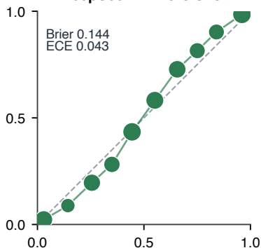
DeepSeek-V4 zero-shot
