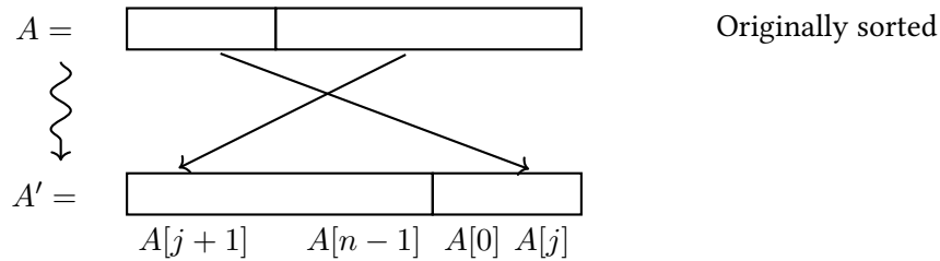
Figure 2.1. A rotated sorted array A' is formed by cyclically shifting blocks of the original sorted array A .
