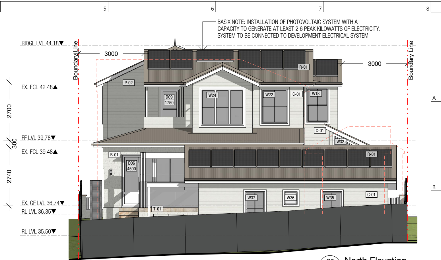
C8 North Elevation SCALE: 1:100
