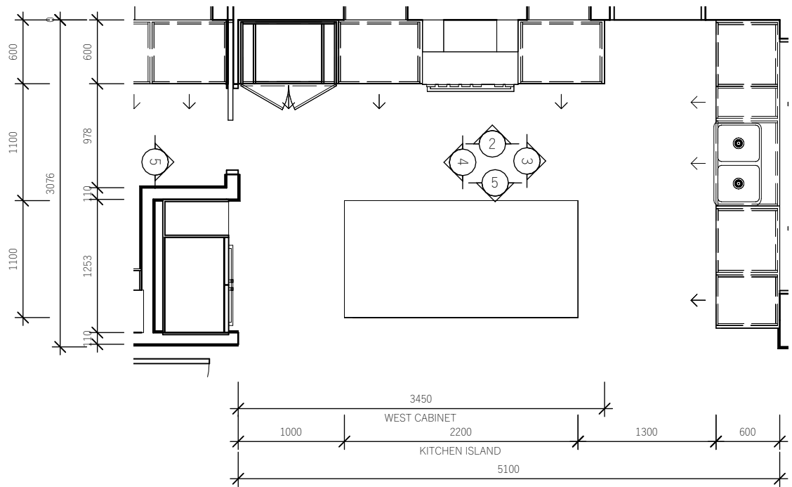
1 KITCHEN FLOOR PLAN SCALE 1 : 50
