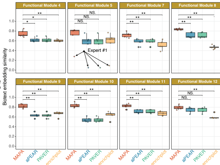
d Functional module annotation comparison
