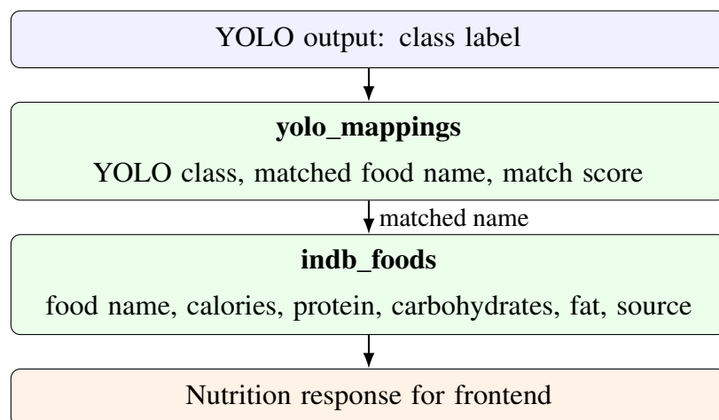
Figure 4.3: Entity relationship used for class-to-nutrition lookup
