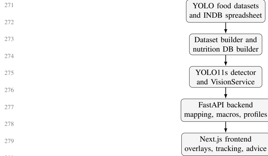
281 Fig. 1. System architecture for nutrition-aware Indian food recognition.
