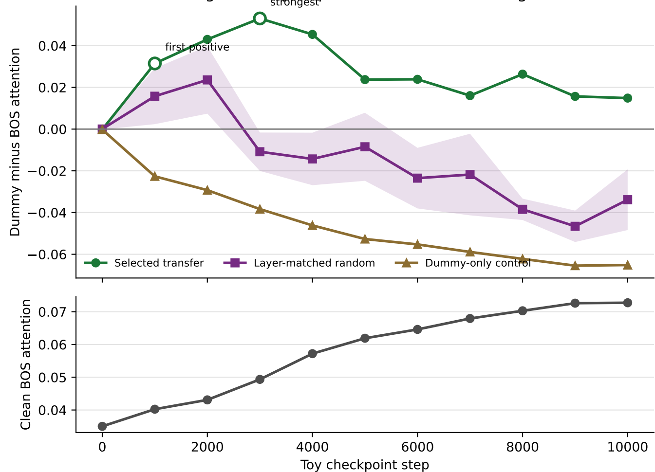
Figure 7. Toy-to-pretrained relocation bridge
