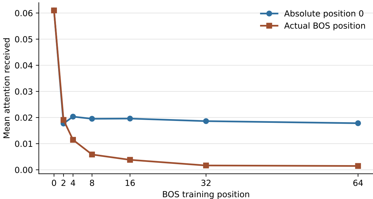
Figure 2. BOS position sweep in toy training
