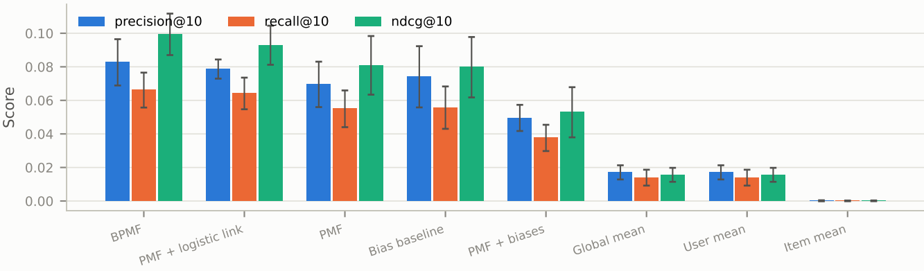
Top-10 ranking quality
