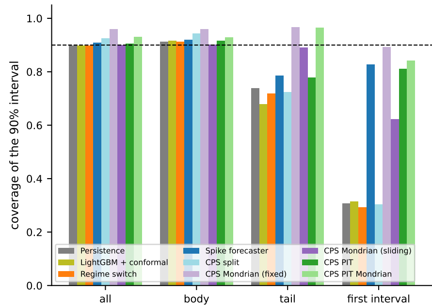
Test window: 90% interval coverage and width by regime (tail = realised price outside the train 5-95% band)
