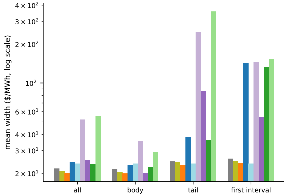
Test window: 90% interval coverage and width by regime (tail = realised price outside the train 5-95% band)
