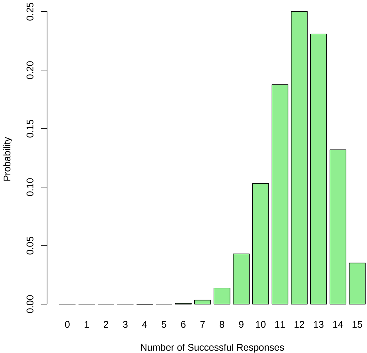
Binomial Distribution ( n=15 , p=0.8 )
