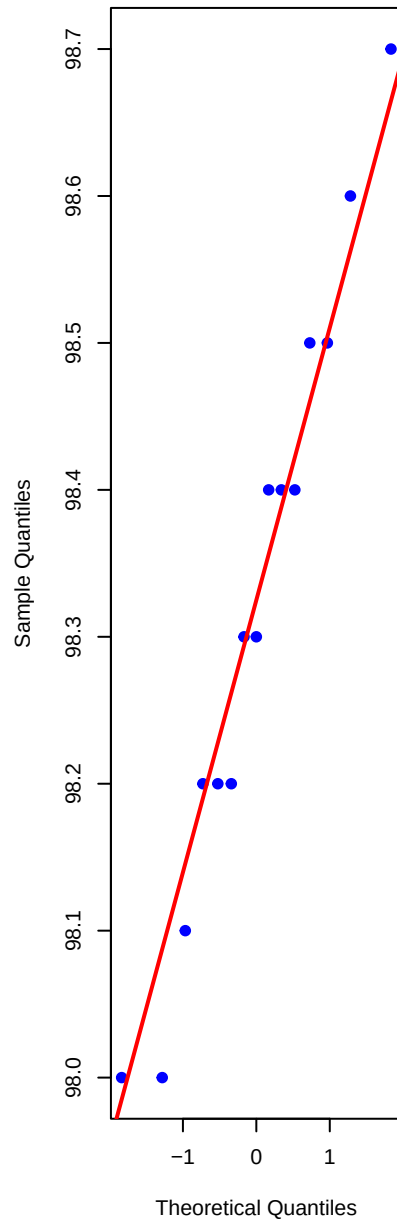
Q-Q Plot
