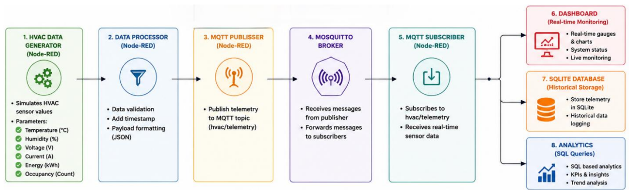
Figure 5.1: HIGH LEVEL DIAGRAM OF THE SYSTEM
