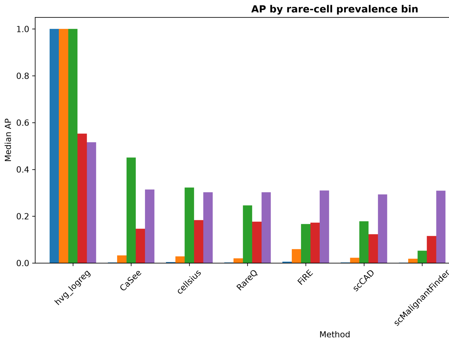
Figure 8: Figure 4. Average precision stratified by rare-cell prevalence.
