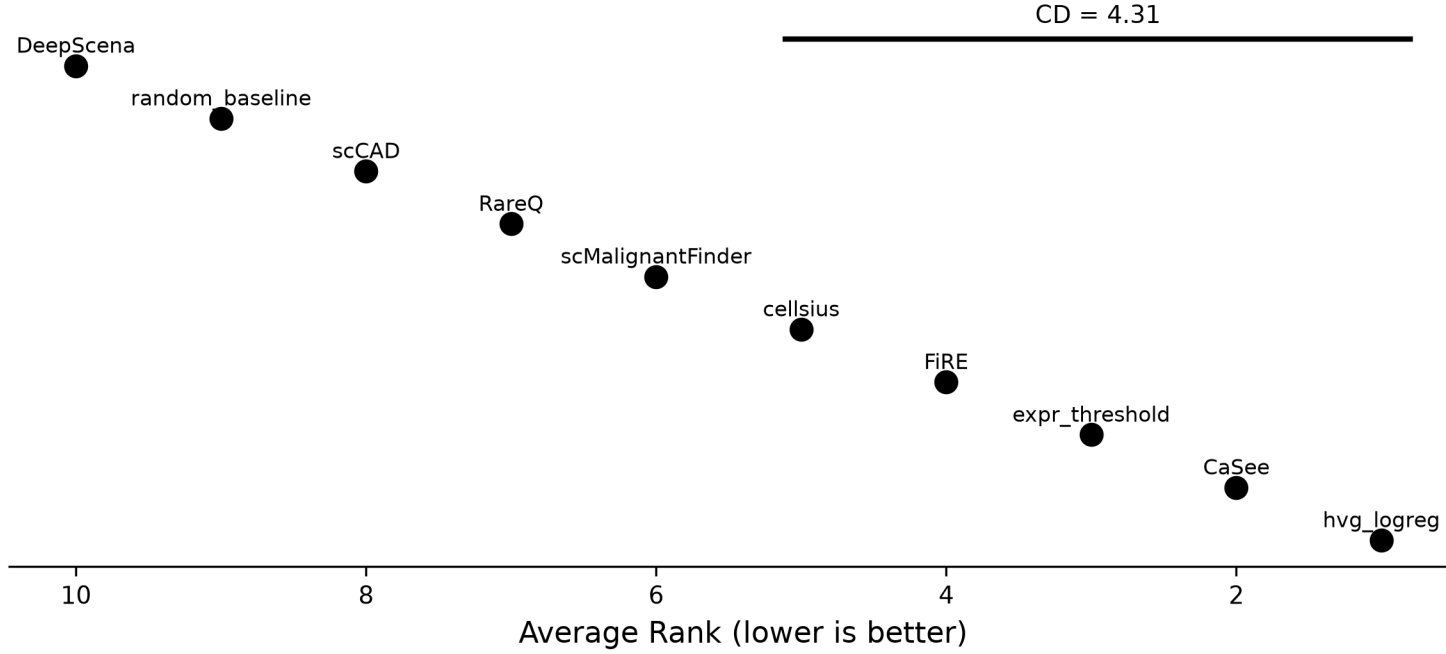
Figure 7: Figure 3. Critical difference diagram for method ranking.
