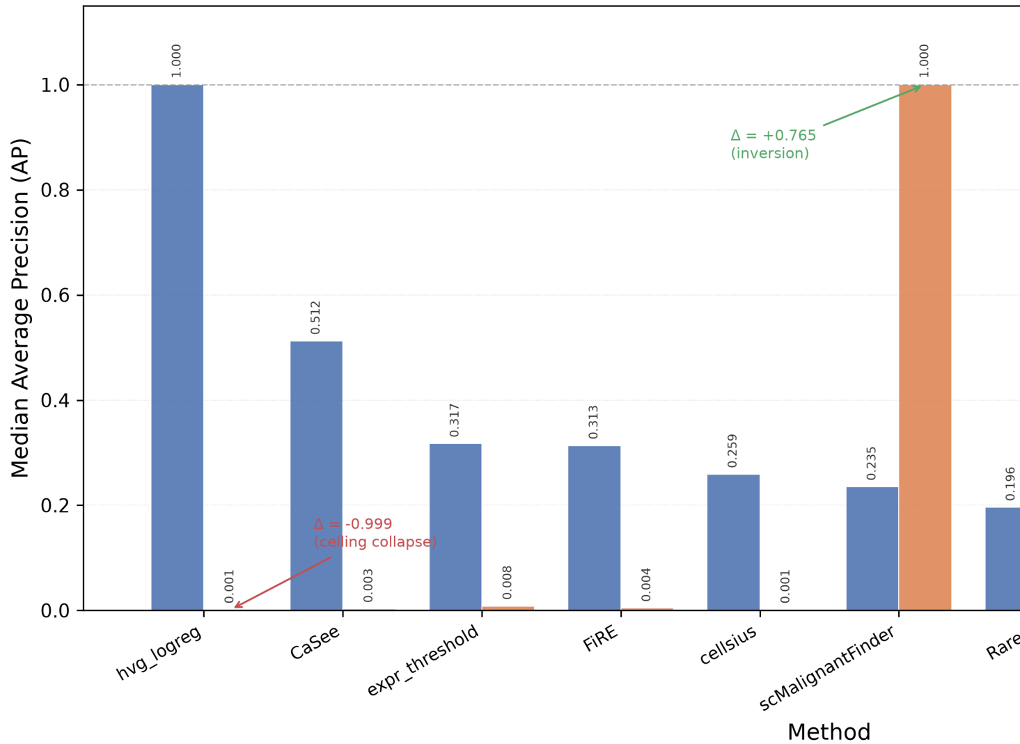
Figure 11. Track F (Intra-lineage) vs Track A (Inter-lineage) Malignant epithelial detection — crc_lee, N = 15 units (3 prev
