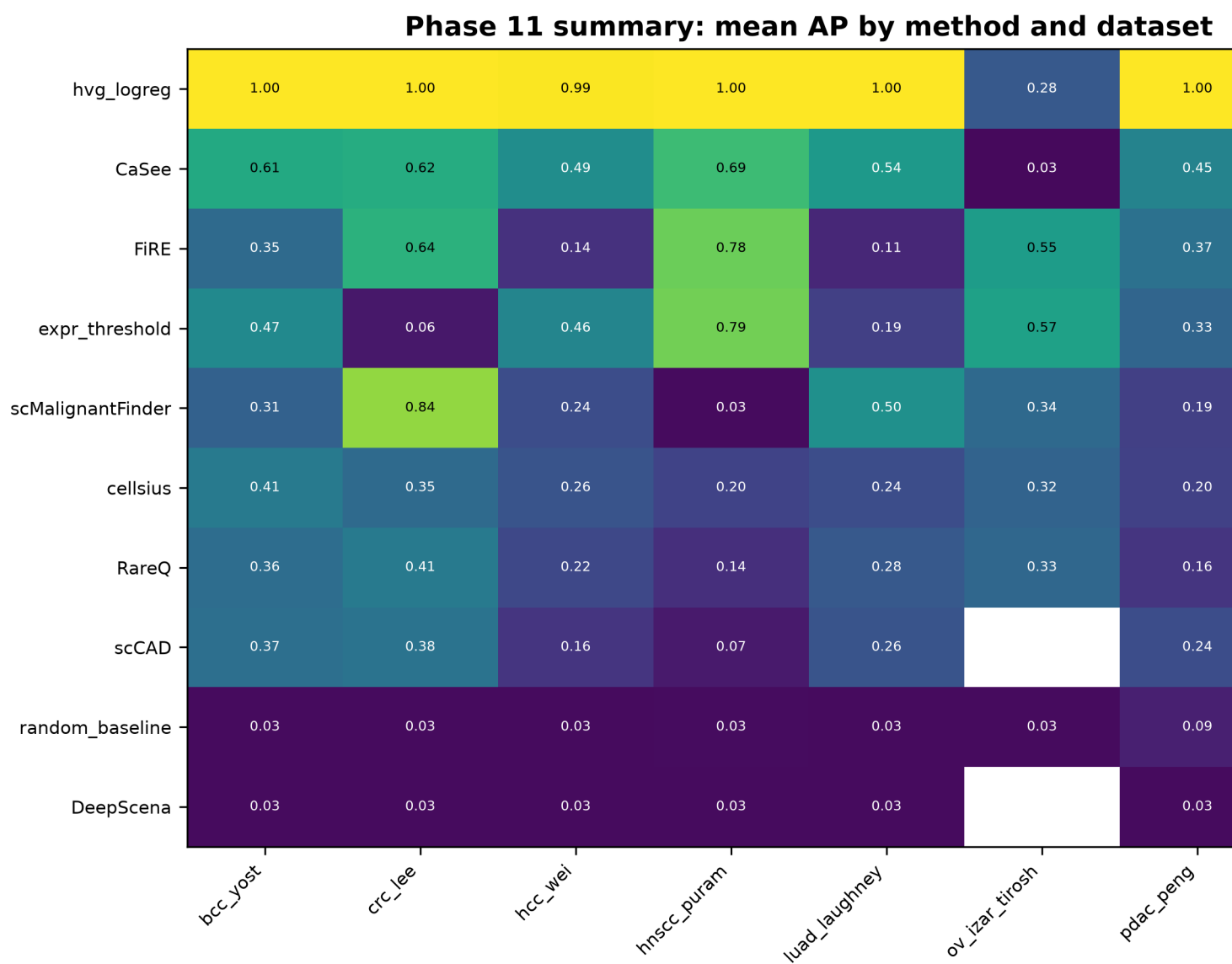
Figure 1: Figure 0. Phase 11 summary heatmap: mean AP by method and dataset.
