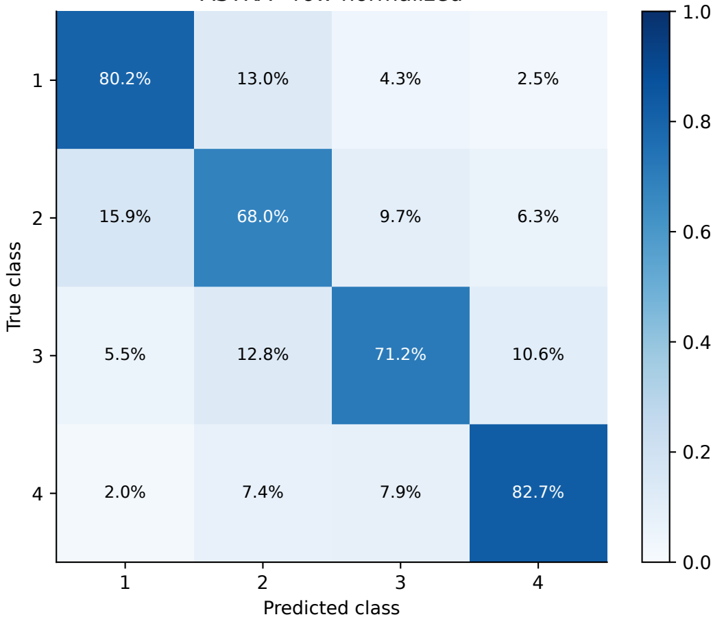
ASTRA · row-normalized
