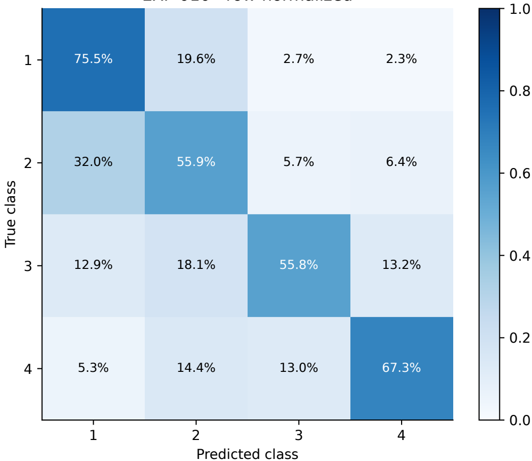
EXP-010 · row-normalized
