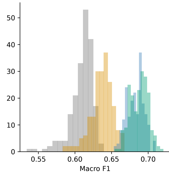
25 shots/class
