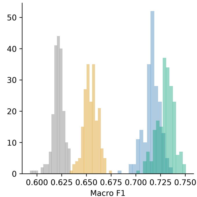
100 shots/class
