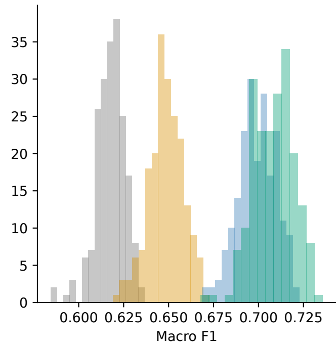
50 shots/class
