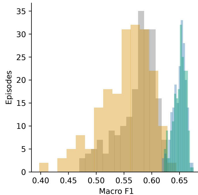
5 shots/class
