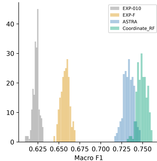
200 shots/class
