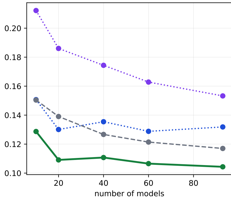
Unified estimation of the full score matrix (SUITE): one ensemble beats the best score-only predictor across all three levers
