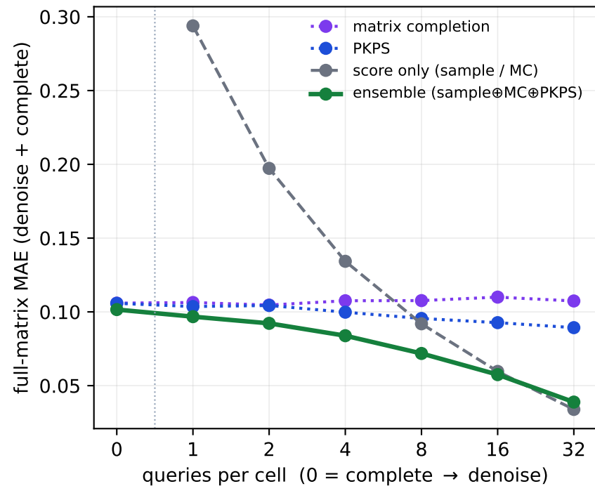
Unified estimation of the full score matrix (SUITE): one ensemble beats the best score-only predictor across all three levers
