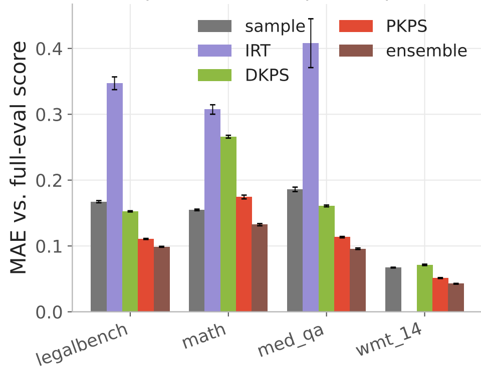
(a) per dataset, unpaired ( \rho = 0 )
