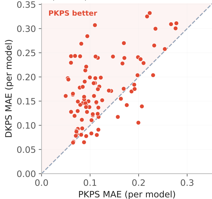
(b) unpaired, per model: PKPS < DKPS for 82%
