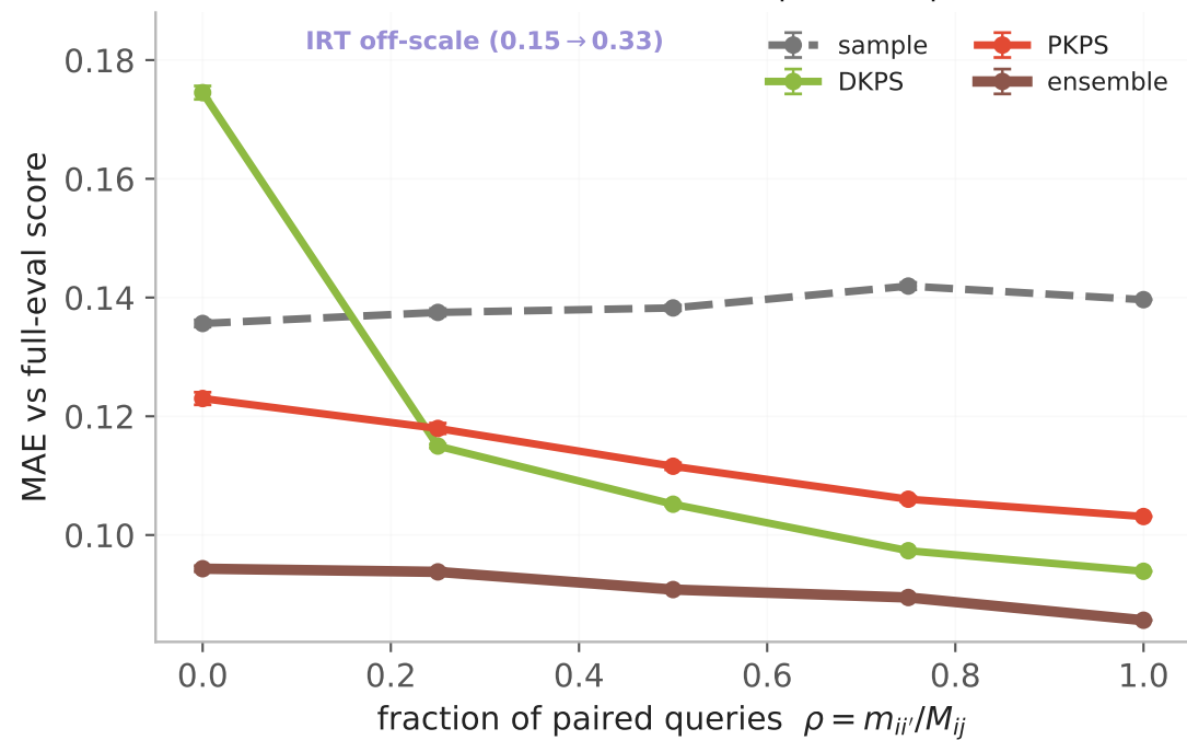
(a) the cliff: PKPS holds as queries unpair
