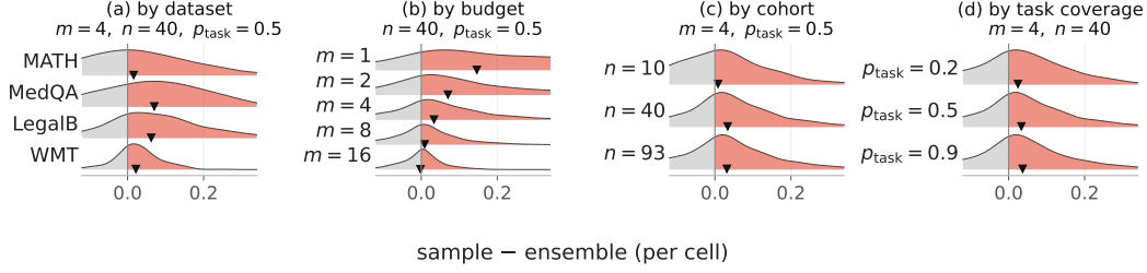
Figure 4: Conditional breakdown of the query-efficiency win. Per-cell \Delta = sample – ensemble MAE ( \Delta > 0 , red = win) by dataset, budget m , cohort n , and coverage p_{\text{task}} , other levers at their sweep median. Broad but tail-driven; the per-row mean ( \blacktriangledown ) is positive throughout.
