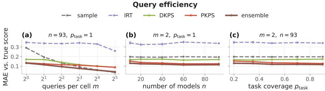
Figure 3: Query efficiency . Each model answers m unpaired queries per observed cell; predict its true full-eval score (MAE, \pm 1 SEM). PKPS (red) and the ensemble (brown) denoise far below the raw sample (grey) at small budgets and across cohort (b) and coverage (c); DKPS (green) trails on unpaired queries, and IRT (purple) is poorly identified without a shared item block.
