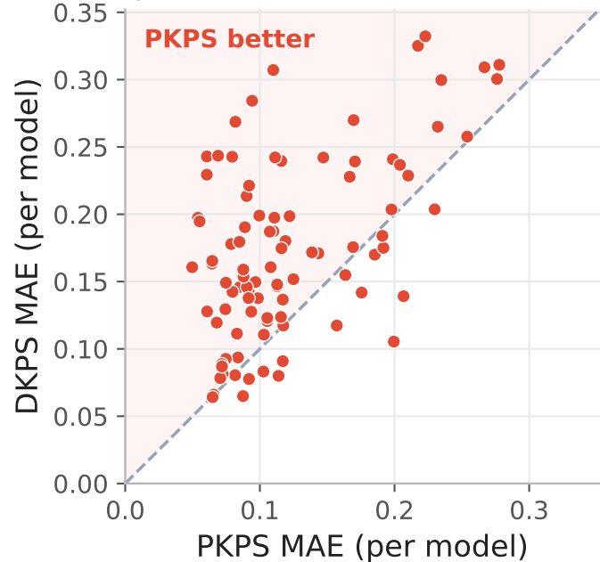
(b) per model: PKPS < DKPS for 82%
