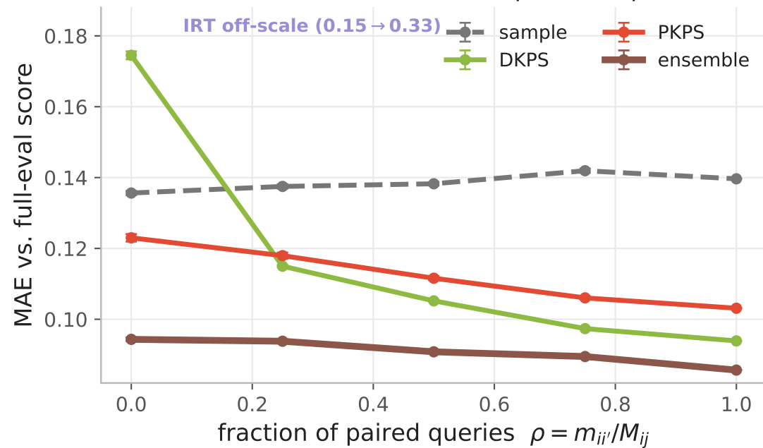
(a) the cliff: PKPS holds as queries unpair
