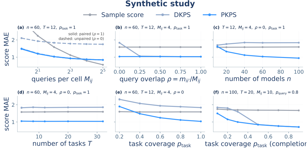
Figure 2: Score MAE on the synthetic benchmark ( \pm 1 SEM over 50 seeds; DKPS light blue, PKPS bright blue, sample score gray; fixed parameters in each panel title). (a–e) Query-efficient evaluation: every observed cell is measured with M_{ij} noisy queries and we predict its true score, as a function of the budget M_{ij} at paired ( \rho=1 , solid) and unpaired ( \rho=0 , dashed) designs (a), the cross-model overlap \rho (b), the cohort size n (c), the number of tasks T (d), and the task coverage \rho_{\text{task}} (e). (f) Score completion of held-out cells as a function of task coverage; the gray line is the task mean of observed scores (no sample score exists for a held-out cell).
