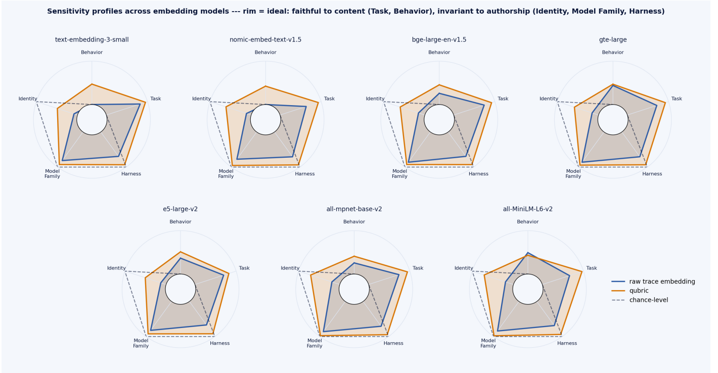
Figure 1: Sensitivity radars across seven embedders. Outside = desirable. Raw embeddings (navy) are authorship-dominated; qubric (amber) collapses Identity / Model family / Harness to chance while holding Task and Behavior.
