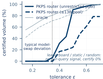
(b) The guarantee: median volume at P(\text{dev} > \epsilon) \leq 10\%
