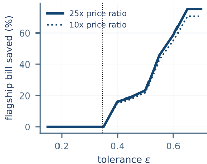
(c) The savings ( \leq 13\text{B} substitutes)
