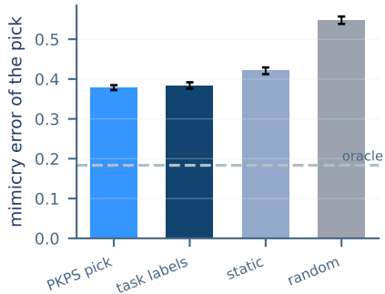
(a) The pick: label-free, no task metadata
