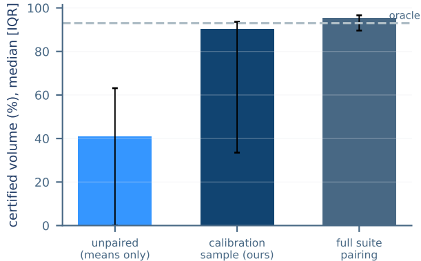
(a) Confidence needs exact pairs; the calibration sample suffices
