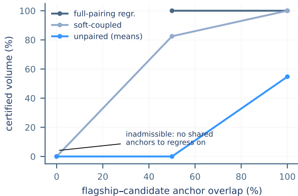
(b) Controlled ablation: coupling must be exact (HELM, fixed cache)
