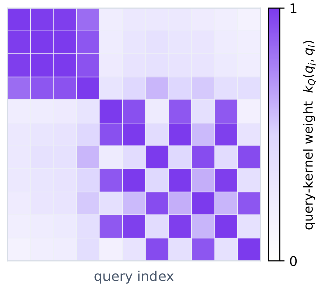
(c) PKPS · k_Q = \text{RBF}
