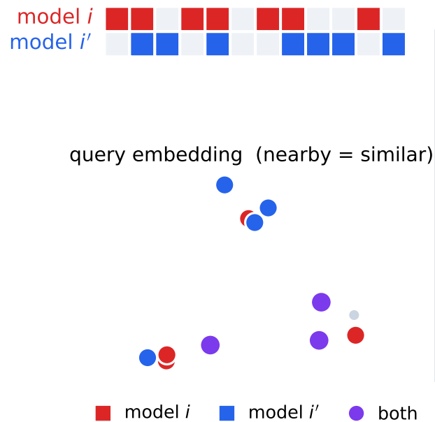
(a) answered queries
