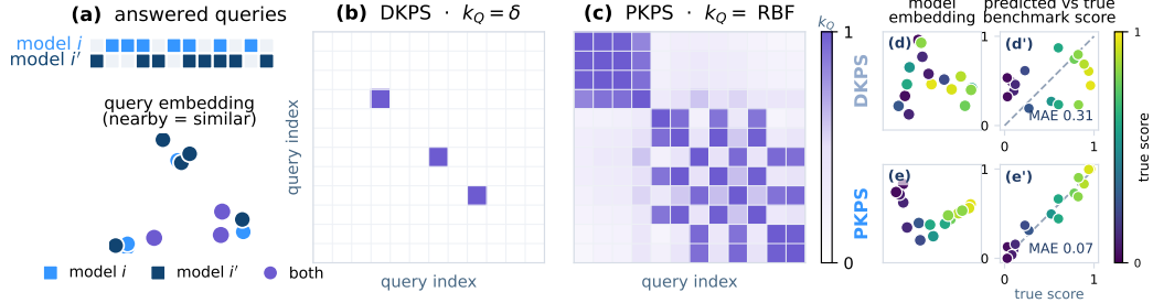
Figure 1: An illustration of the difference between the Product Kernel Perspective Space (PKPS) and the Data Kernel Perspective Space (DKPS). (a) Top: two models respond to different sets of queries. Bottom: queries represented as vectors, colored by which model has responded to them. (b) The query kernel used by DKPS. Only information from queries both models have responded to is included. (c) The query kernel weighs query similarity in the embedding space. (d–e') A benchmark prediction example. Left: each dot is a model colored by its benchmark score. Right: true benchmark score versus predicted benchmark score. Restricted to the rare shared queries, DKPS (top) is noisy and correlates poorly with benchmark score (MAE 0.31). PKPS (bottom) leverages unpaired queries and the is highly correlated with true score (MAE 0.07).
