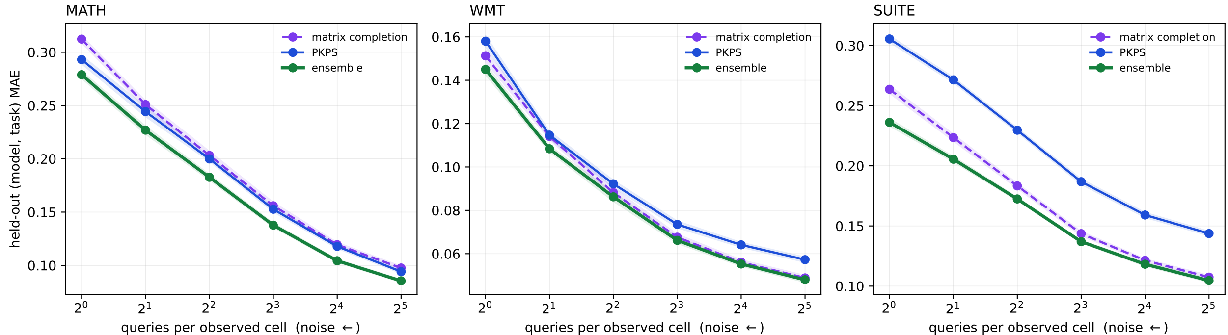
RD2 under evaluation noise: the PKPS ensemble overtakes matrix completion as cells get noisier
