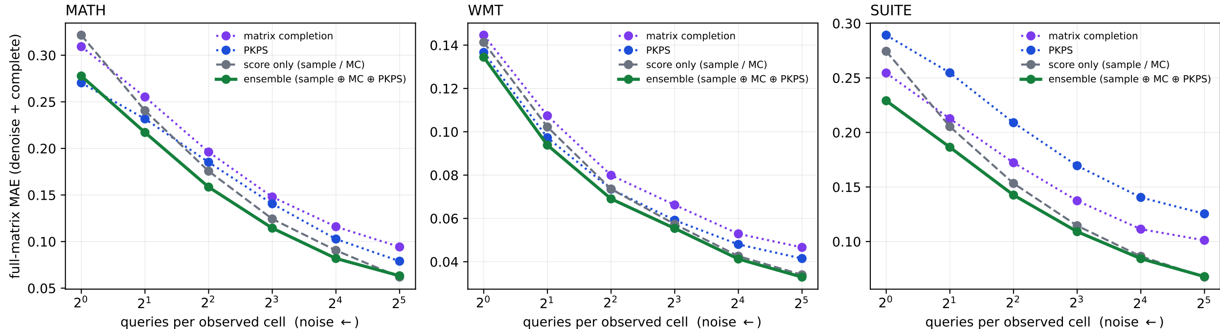
Unified estimation of the full score matrix: one sample \oplus MC \oplus PKPS ensemble beats the best score-only predictor, by more as queries shrink
