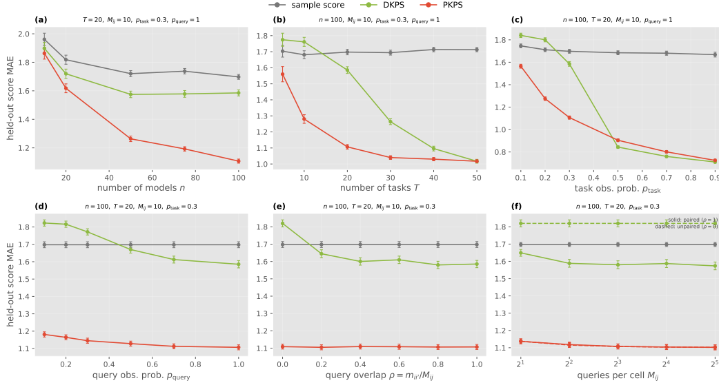
Figure 2: Synthetic study (held-out score MAE, \pm 1 SEM over 50 seeds). DKPS (identity query kernel, green) vs. PKPS (RBF, red), with the score-only sample baseline (task mean, gray) as a floor. Each panel sweeps one parameter with the rest fixed (shown in its title): (a) cohort n , (b) tasks T , (c) task coverage p_{\text{task}} , (d) query coverage p_{\text{query}} , (e) cross-model overlap \rho = m_{ij}/M_{ij} , (f) per-cell query budget M_{ij} at paired ( \rho=1 , solid) and unpaired ( \rho=0 , dashed). \text{PKPS} \leq \text{DKPS} throughout; the gap is small when queries are paired (a–c) and large when unpaired or sparse (d–f). In (e) DKPS collapses to the sample floor as overlap vanishes while PKPS stays flat; in (f) PKPS keeps improving with budget even fully unpaired while unpaired DKPS gains nothing.
