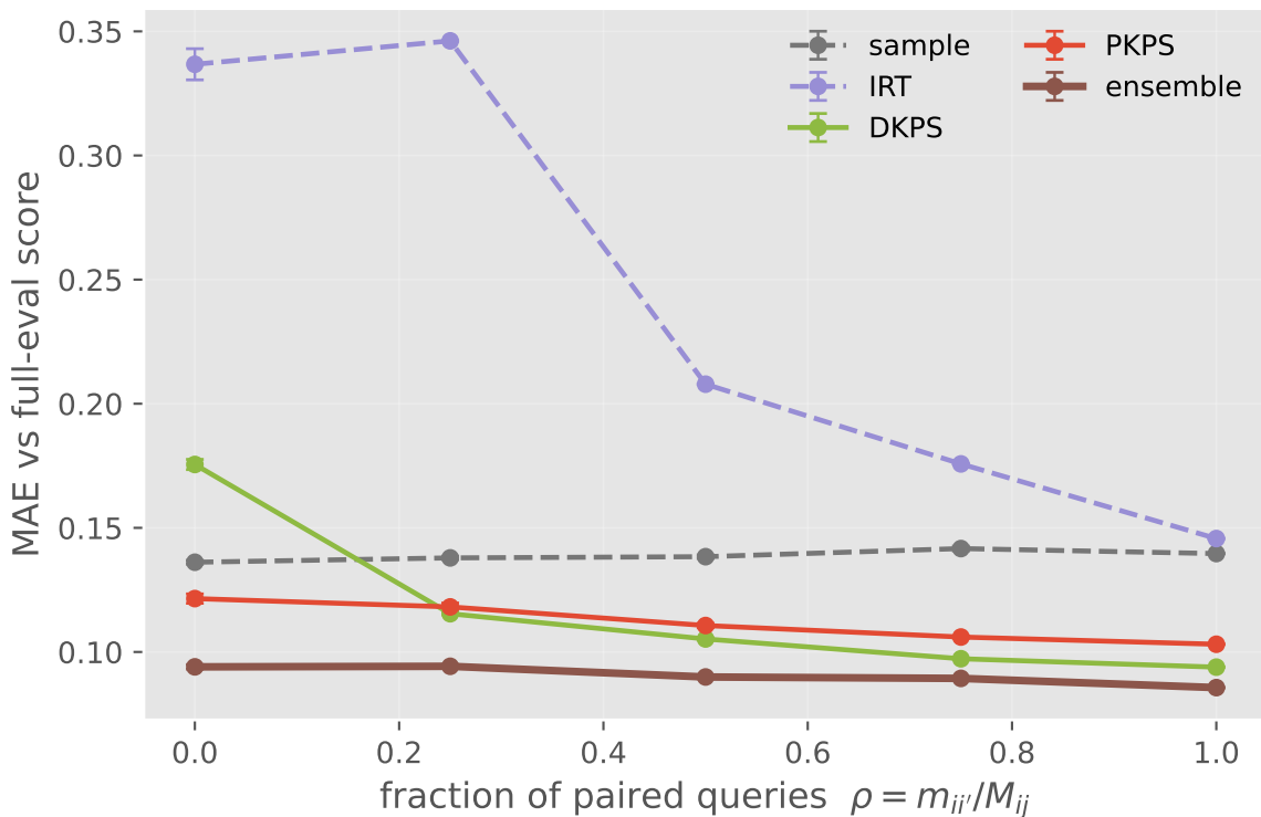
Unpaired evaluation (suite, budget M_{ij} = 4 queries/cell): DKPS and IRT collapse as queries unpair; PKPS holds
