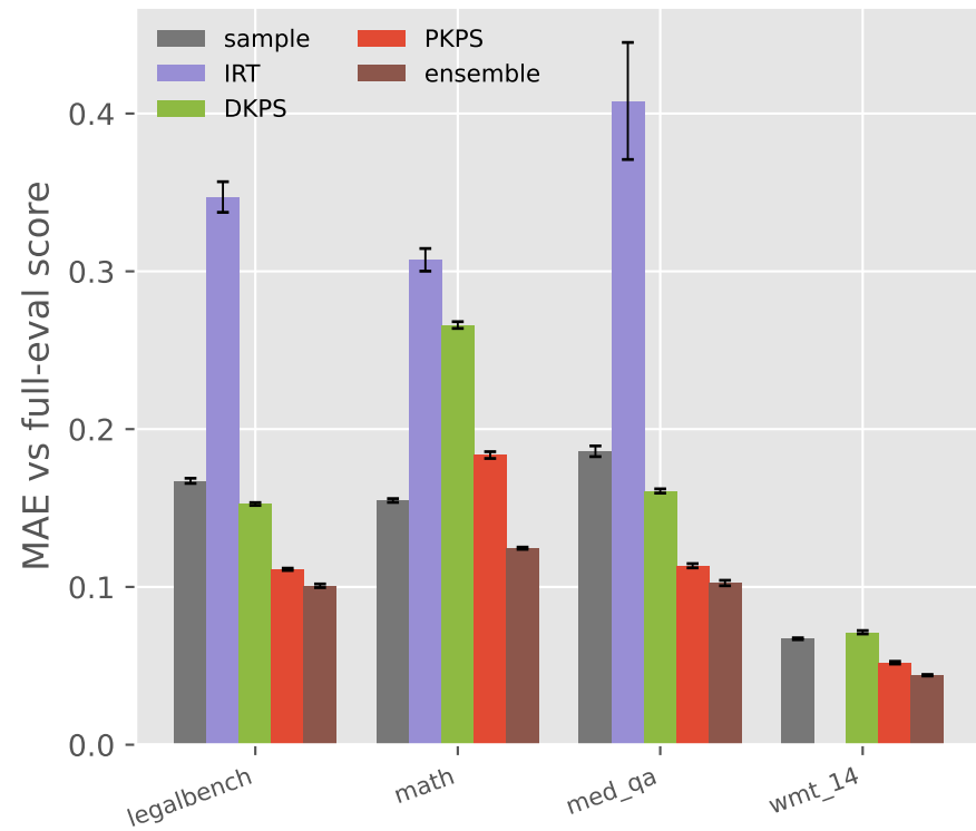
(a) per dataset, unpaired ( p = 0 )
