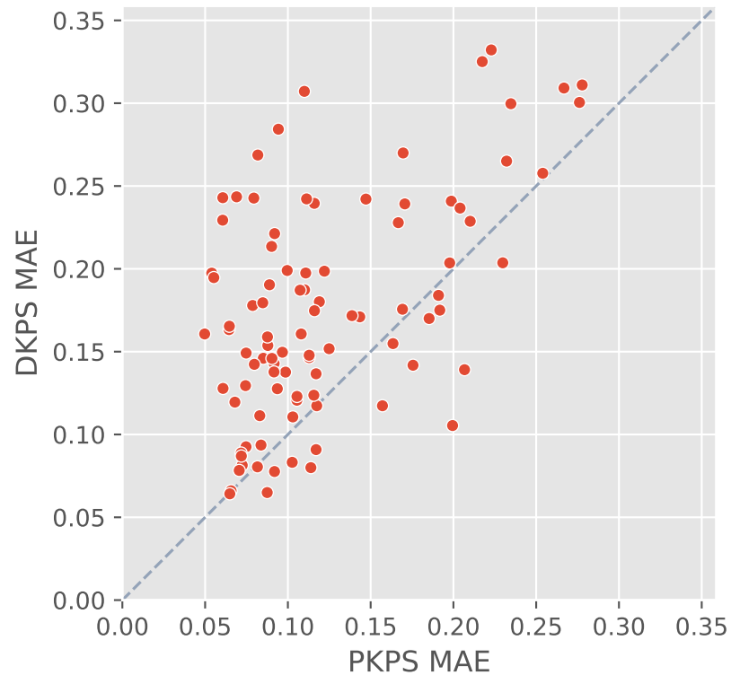
(b) per model, unpaired: PKPS < DKPS for 82%
