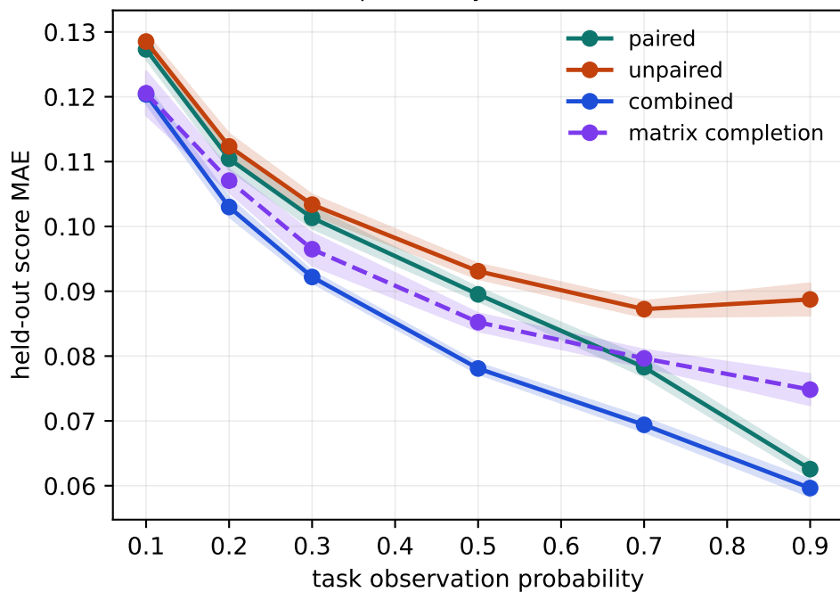
(a) task observation probability
