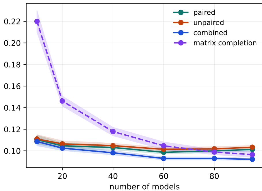
(b) number of models
